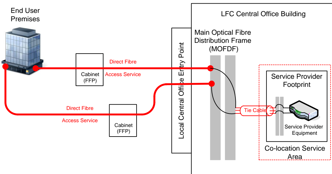
Single Central Office redundancy with diverse route, diverse access to End User Premises and diverse access to Central Office
